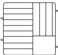
Plate Rack w/6 Extenders No. PM1211-6 Plate - D10¼ to D11⅝ Max. H1⅝, Cap. 12 1 pc./16# • 3.3 cu.ft.
