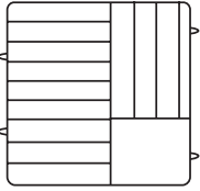
Plate Rack w/5 Extenders No. PM1211-5 Plate - D9 \frac{3}{16} to D10 \frac{3}{4} Max. H1 \frac{1}{4} , Cap. 12 2 pc./27# • 5.5 cu.ft.
