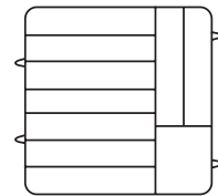
Plate Rack w/6 Extenders No. PM0912-6 Plate - D11¼ to D12½ Max. H2⅝, Cap. 9 1 pc./14# • 3.3 cu.ft.
