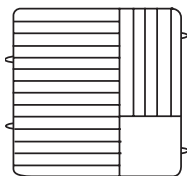
Plate Rack w/6 Extenders No. PM1911-6 Plate - D10¼ to D11⅝ Max. H1⅝, Cap. 19 1 pc./14# • 3.3 cu.ft.
