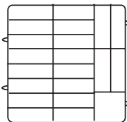
Plate Rack w/3 Extenders No. PM2006-3 Plate - D4 \frac{3}{4} to D6 \frac{1}{2} Max. H2, Cap. 20 2 pcs./11# • 4.2 cu.ft.
