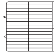
Plate Rack w/4 Extenders No. PM3208-4 Plate - D7 \frac{7}{8} to D8 Max. H1, Cap. 32 2 pcs./12# • 4.3 cu.ft.
