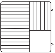
Plate Rack w/4 Extenders No. PM2110-4 Plate - D8 \frac{3}{4} to D9 \frac{3}{16} Max. H1, Cap. 21 2 pcs./14# • 4.3 cu.ft.
