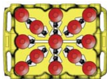
Adjustable Dish Caddy No. ADC-14 14 post dividers 13 stacks holds 4 1 / 2 - 5 1 / 2 plates L40 W30 H31 1 / 16 1 pc./82.25# • 22.23 cu.ft.
