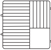
Plate Rack w/5 Extenders No. PM2011-5 Plate - D10 to D10 \frac{3}{4} Max. H1, Cap. 20 2 pcs./27# • 5.5 cu.ft.
