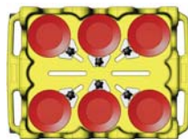
Adjustable Dish Caddy No. ADC-6 6 post dividers 6 stacks holds 8 5 / 8 - 9 1 / 8 plates or 5 stacks holds 9 1 / 8 - 10 5 / 8 plates L40 W30 H31 1 / 16 1 pc./82.25# • 22.23 cu.ft.
